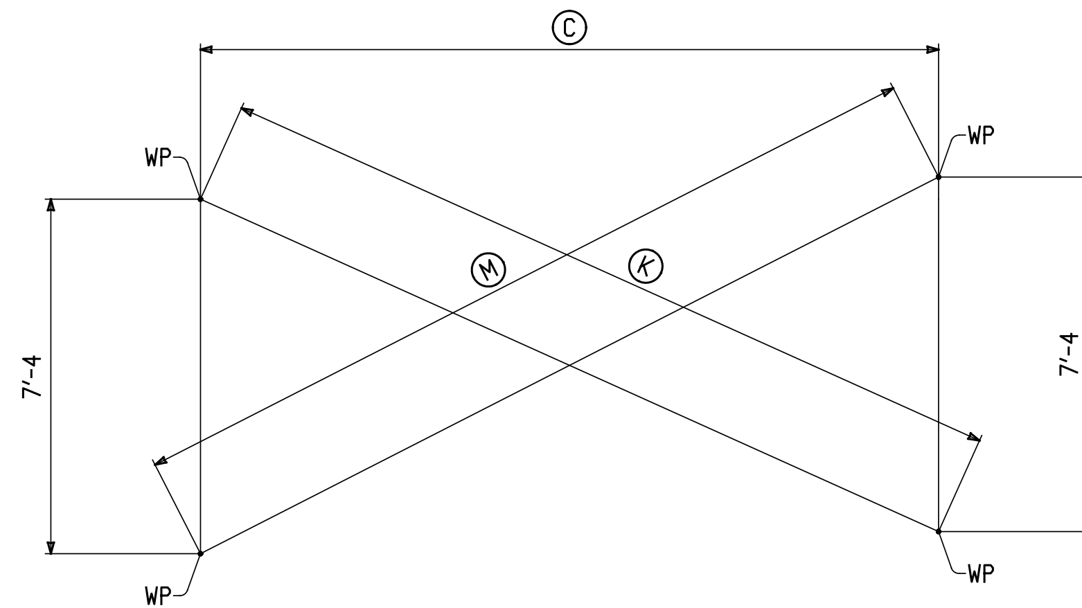
CHECK DIMENSIONS
