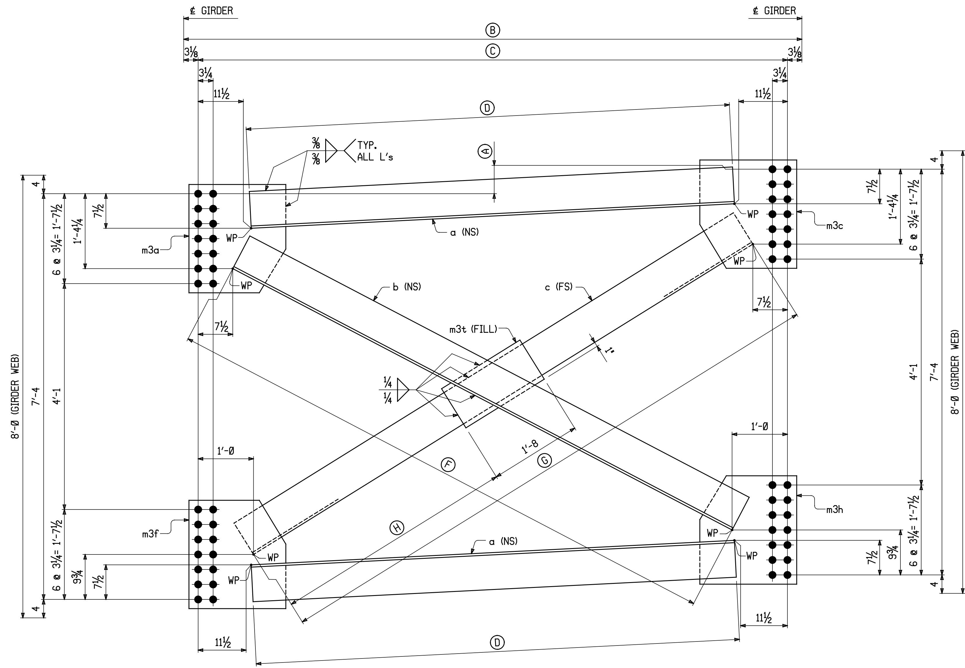
INTERMEDIATE CROSSFRAME
